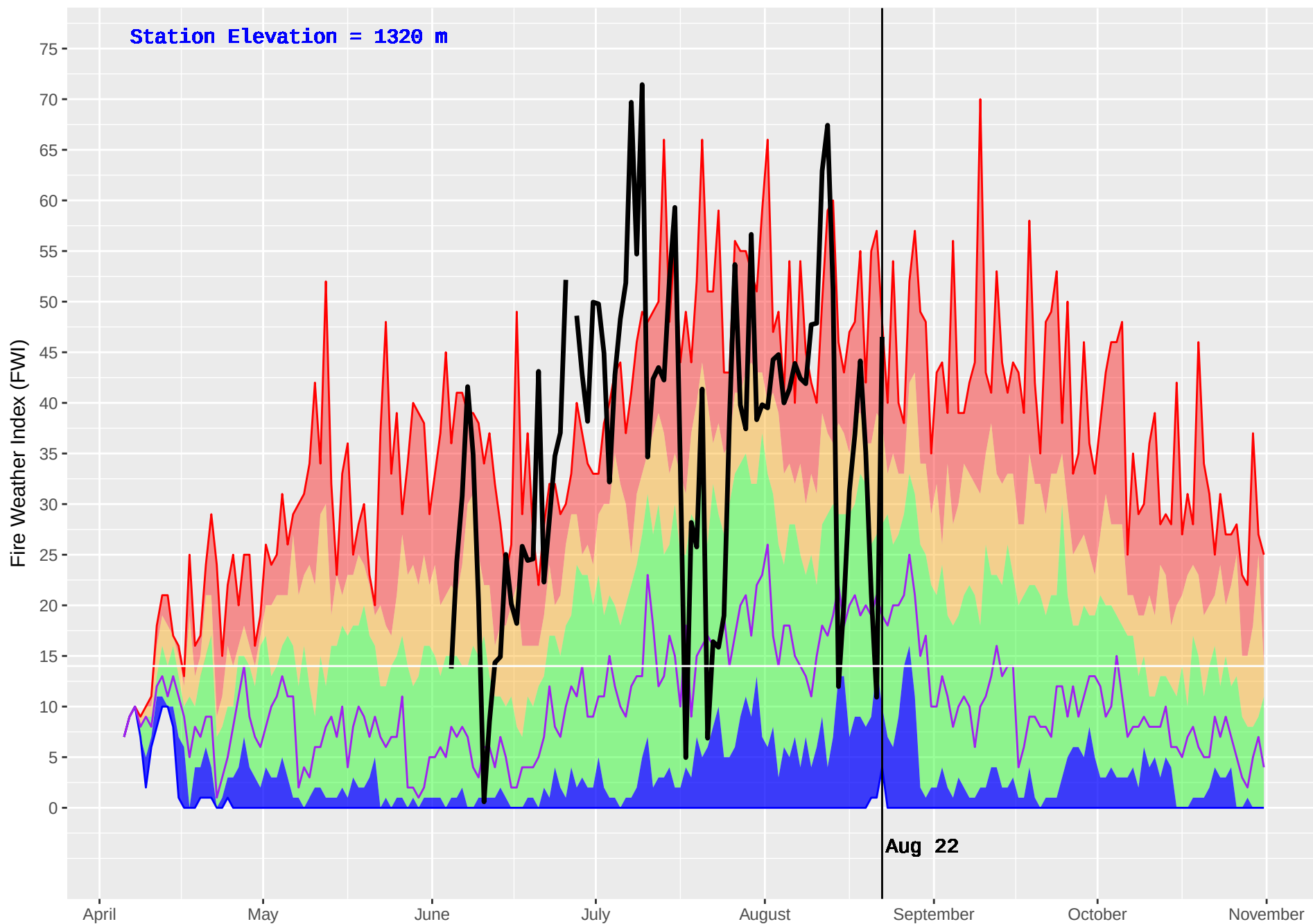
FRENCH BAR (306) : Historical (1979–2016) and Current (2017) Noon Fire Weather Index (FWI)
